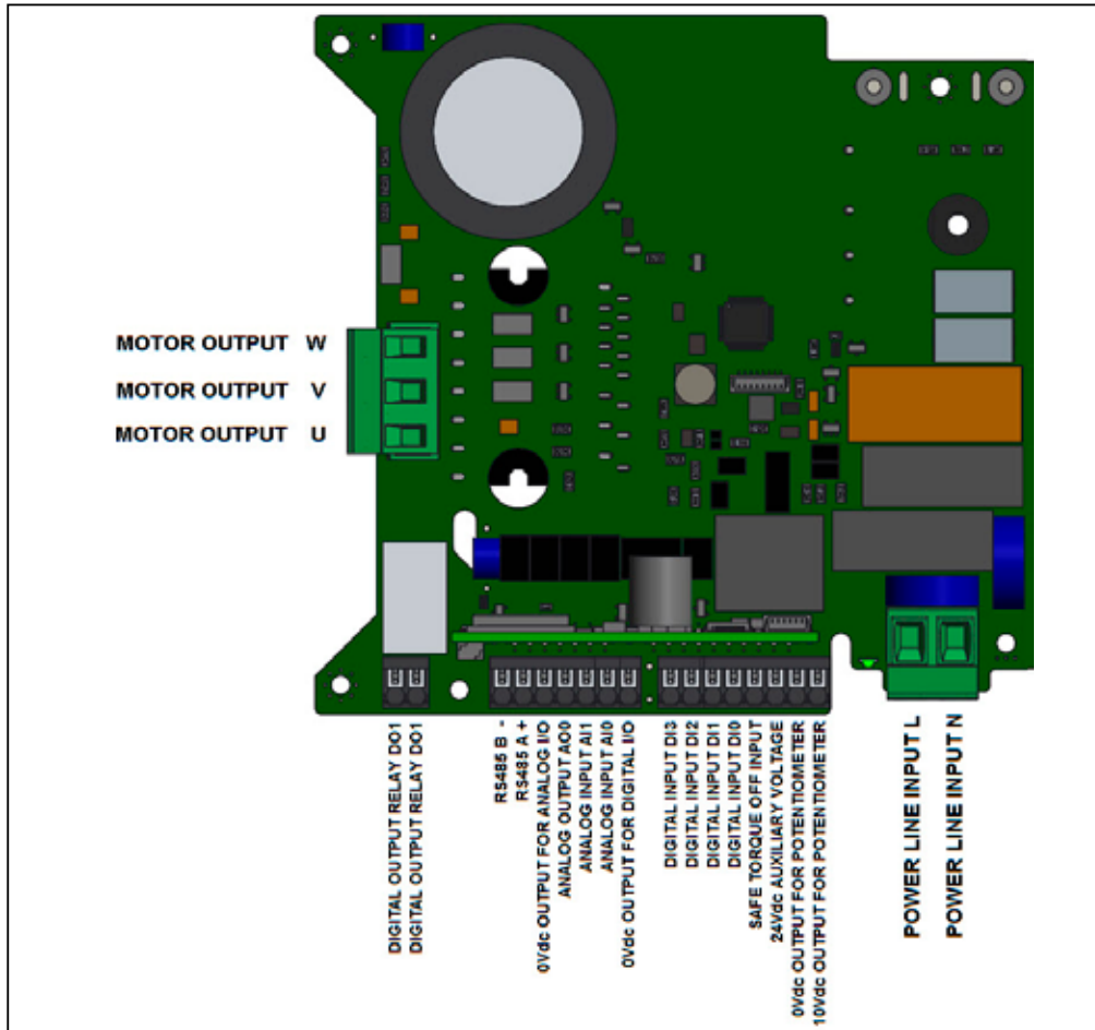
Power Module layout NANO-1.1
