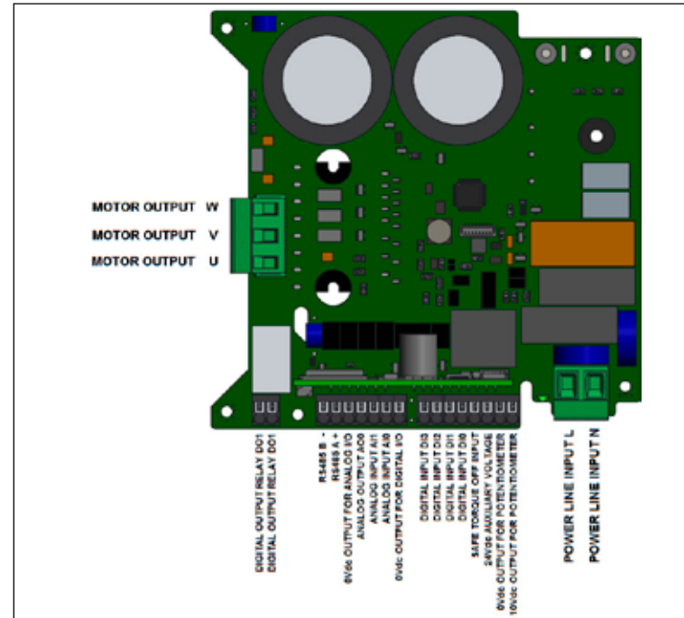
Power Module layout NANO-2.2
