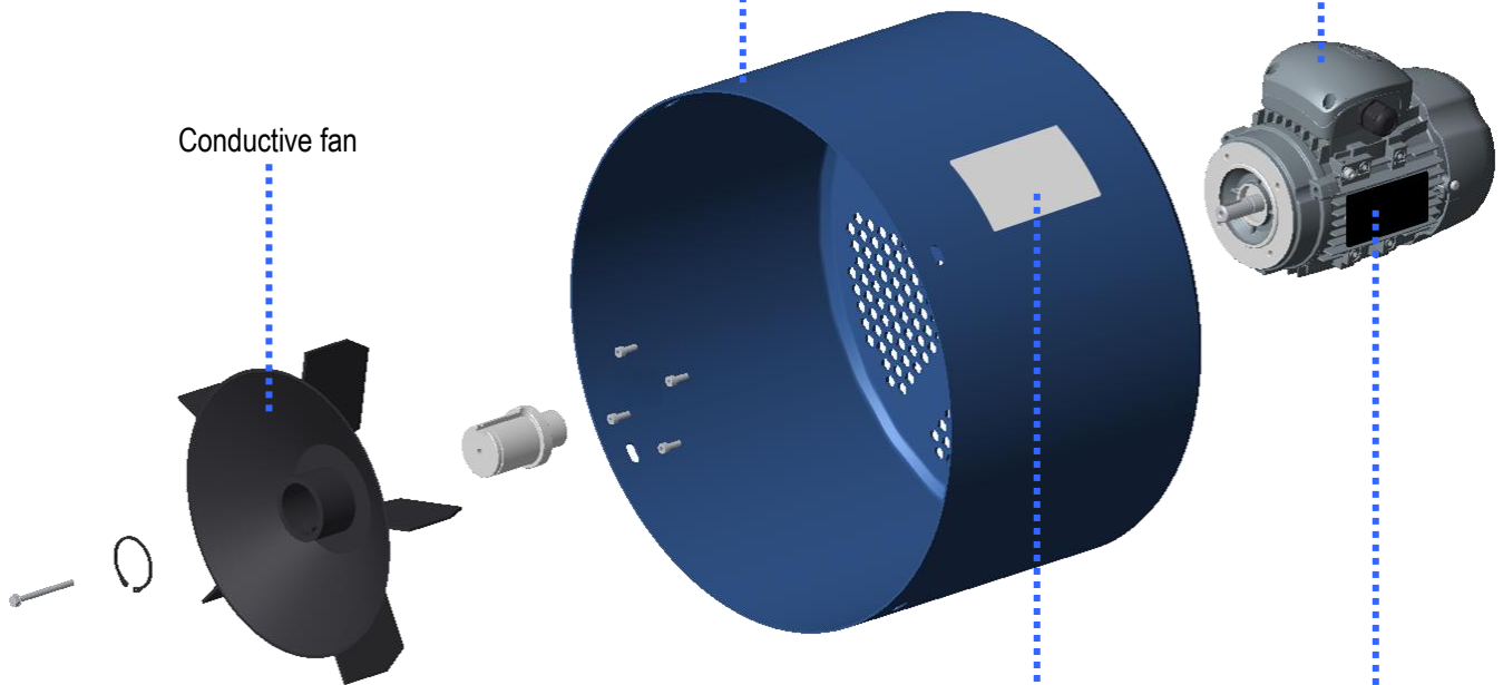
Reinforced fan cover with increased thickness
